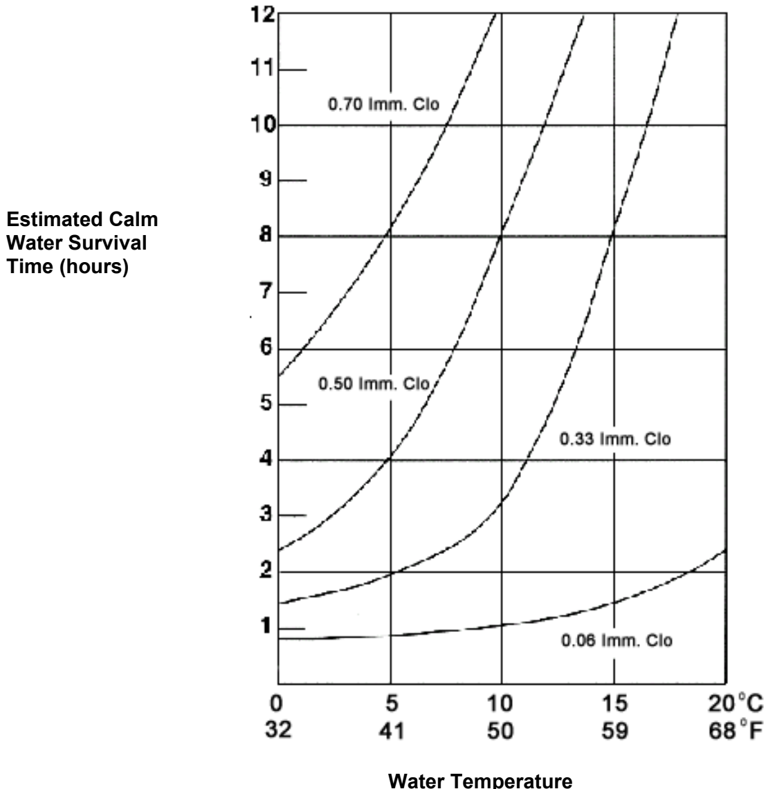
Figure 3. Clo Insulation Graph
