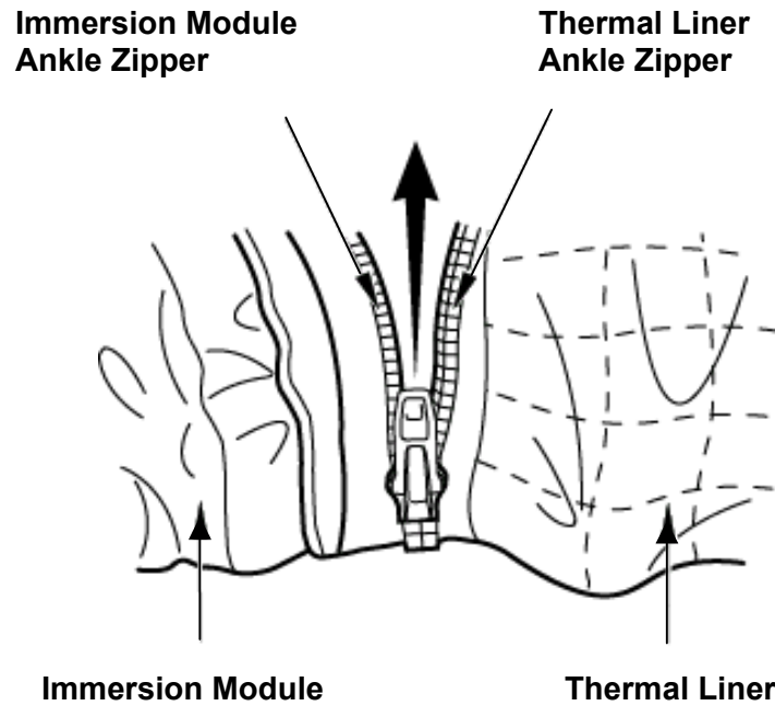
Figure 8. Thermal Liner and Immersion Module Connected at the Ankles
