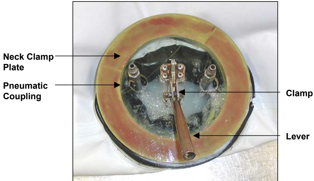
Figure 23. Step d. Suit Leakage Test
