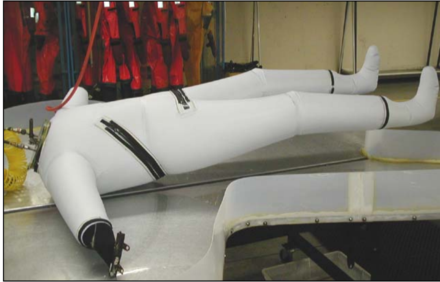
Figure 25. Step f. Suit Leakage Test
