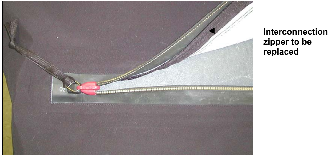
Figure 33. Step a. Interconnection Zipper Replacement
