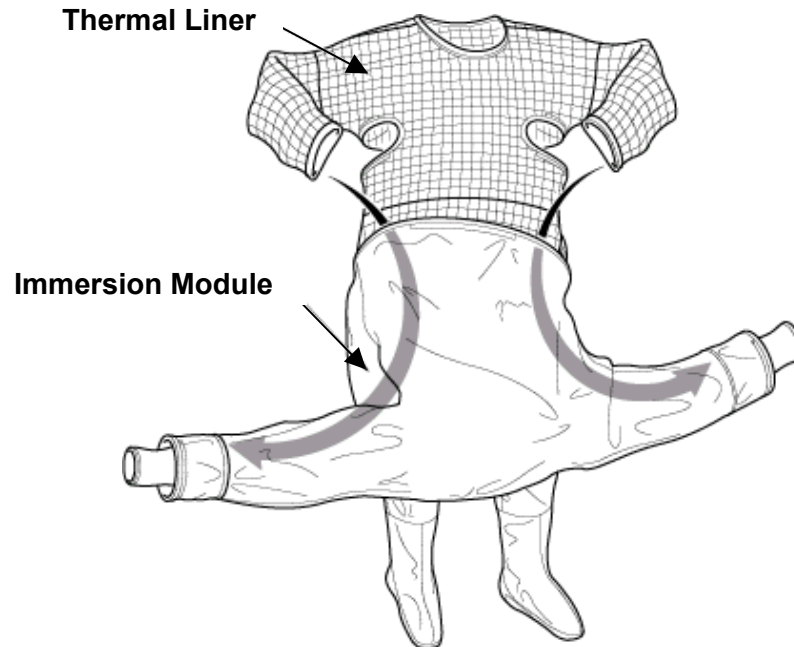
Figure 9. Insertion of the Thermal Liner into the Arm of the Immersion Module
